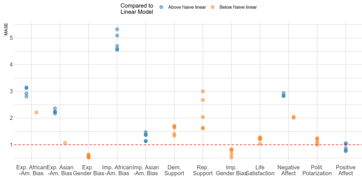
Supplementary Figure 5. Error among top 5 teams in Tournament I versus statistical benchmarks
