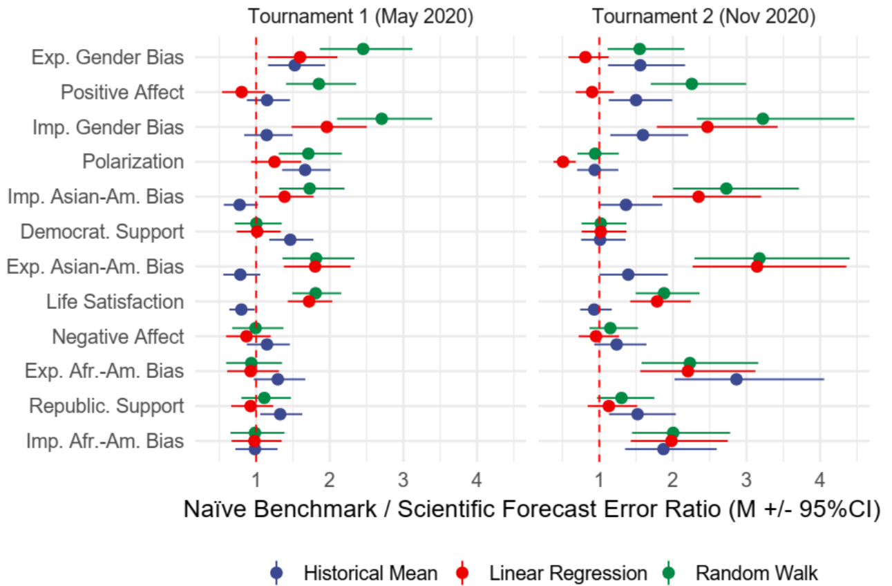
Figure 3. Ratios of Benchmarks against Scientific Forecasts. Scores >1: greater accuracy of scientific forecasts. Scores <1: greater accuracy of naïve benchmarks. Domains are ranked from least to most error among scientific teams in Tournament 1. Estimated means indicate the fixed effect coefficient of a linear mixed model with domain ( k = 12 ) in each tournament ( n_{\text{Tournament 1}} = 86 ; n_{\text{Tournament 2}} = 120 ) as a predictor of benchmark-specific ratio scores nested in teams (observations: n_{\text{Tournament 1}} = 359 , n_{\text{Tournament 2}} = 546 ), using restricted maximum likelihood estimation. To correct for right skew, we used square-root or log-transformed MASE scores, which were subsequently back-transformed when calculating estimated means and 95% confidence intervals. Confidence intervals are adjusted for simultaneous inference of estimates for 12 domains in each tournament by simulating a multivariate t distribution 20 .
