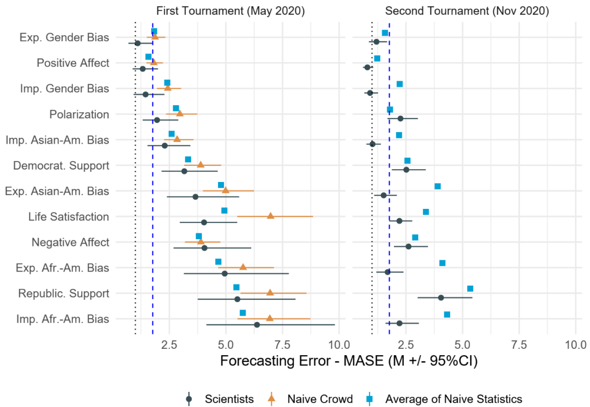
Supplementary Figure 15. Forecasts of scientists, naïve crowd, and the average of statistical benchmarks
