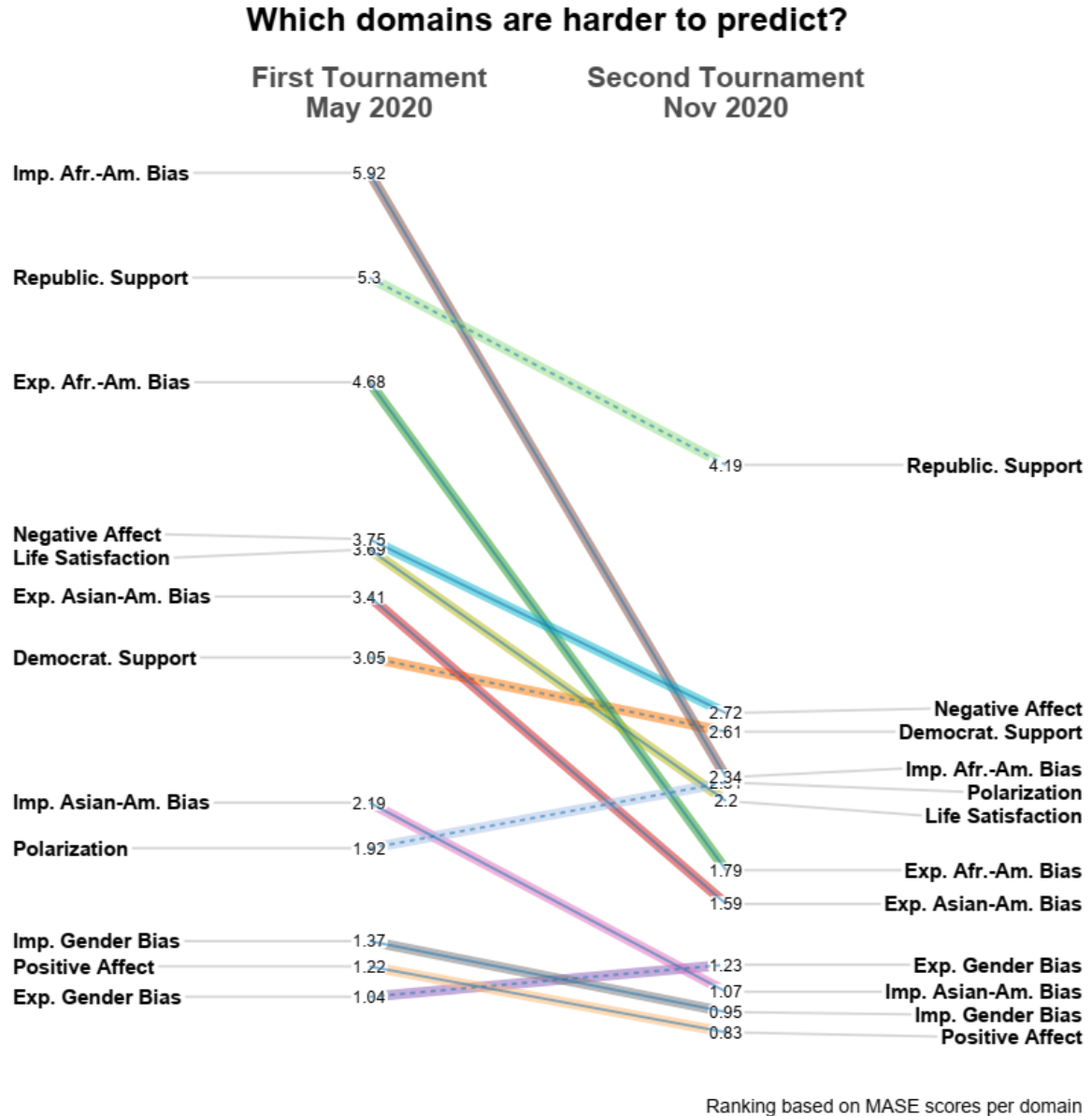
Figure 4. Slope graph showing consistency in the ranking of domains in terms of estimated mean forecasting error across all teams in each tournament, assessed via mean absolute scaled error, from most to least inaccurate forecasts across both tournaments. Solid line = change in accuracy between tournaments is statistically significant ( P < .05 ); dashed line = non-significant change. Significance is determined via pairwise comparisons of \log(\text{MASE}) scores for each domain, drawing on the restricted information maximum likelihood model with Tournament (first or second), domain, and their interaction as predictors of the \log(\text{MASE}) scores, with responses nested in scientific teams ( N_{\text{teams}} = 120, N_{\text{observations}} = 905 ).
